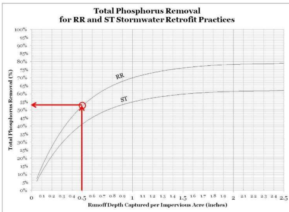
Figure 1 - Retrofit Pollutant Removal Adjustor Curve for Total Phosphorus (TP)
