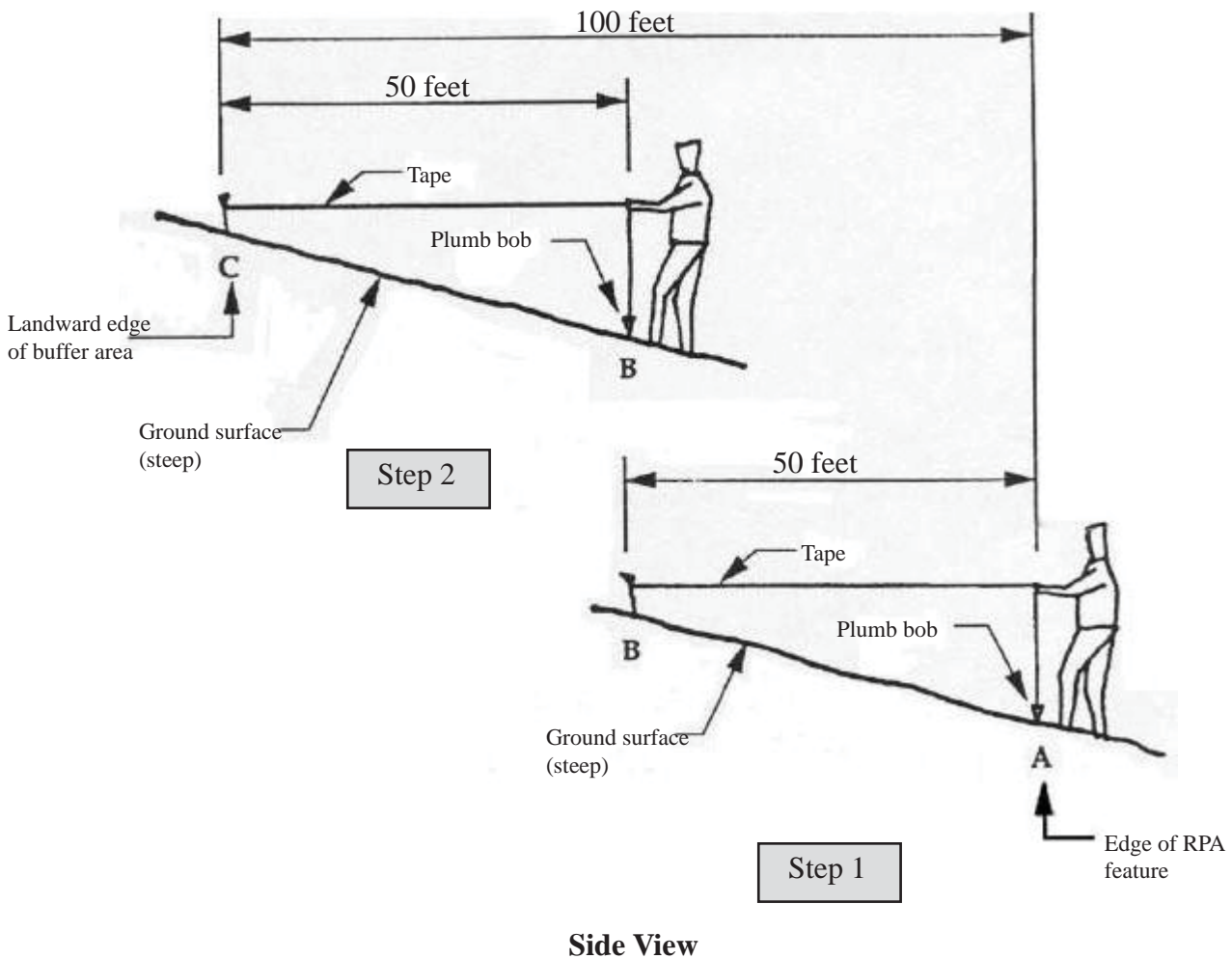
Figure 2 - Measuring along steep slope (Two people)
